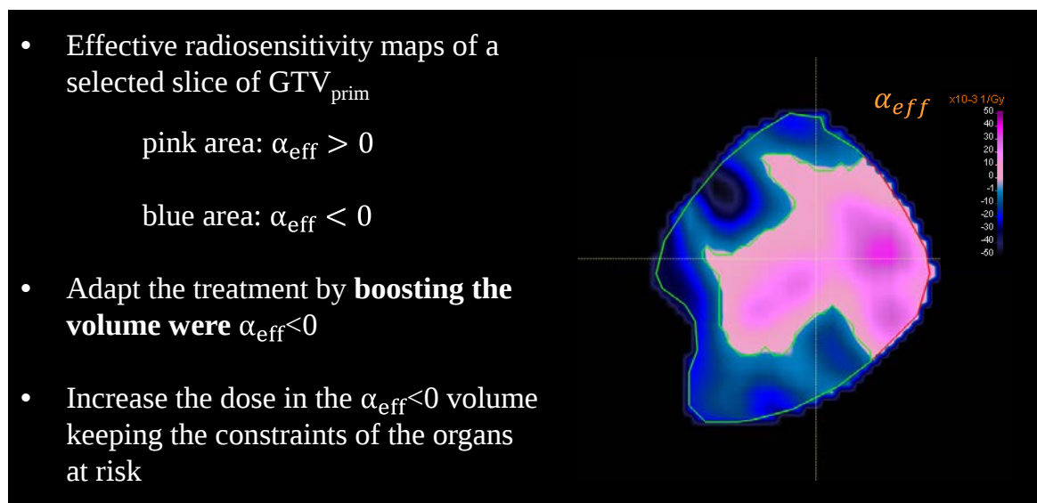
Figure 10. Illustration of the method planned to be used for determining the area that might benefit from a dose boost derived from the calculated map of effective radiosensitivity; the area showing negative values of \alpha_{eff} is identified and delineated as the boost region.
