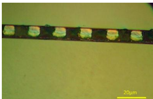
Figure 9. Optical photograph showing, 7.5\mu\text{m} diameter, 20\mu\text{m} Cu/Sn bumps, assembled using capillary self alignment [7].
