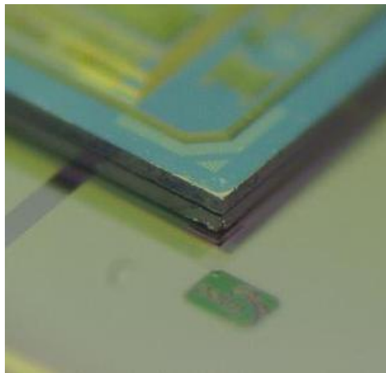
Figure 25. 50 \mu m thin dies bonded on substrate forming a 3 layer stack.
