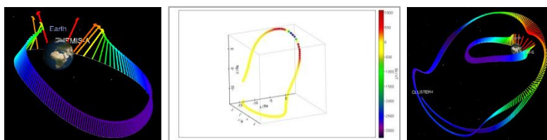
Figure 24: l.t.r: Magnetic field calculated along Themis-A trajectory (CDPP-3DView). Example of the magnetic field visualization (Topcat). Magnetic field calculated along Themis-E and Cluster4 trajectories (CDPP-3DView).
