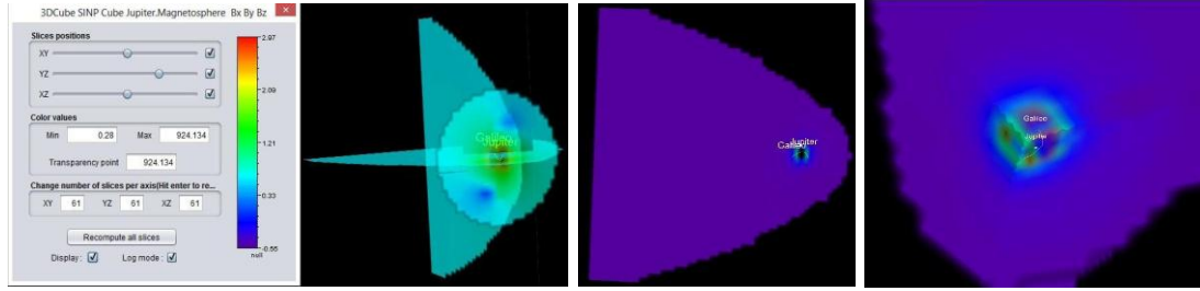
Figure 34: Components and slices of magnetic vector field in the cube -100 < x < 100 Rj with calculateCubeJupiter . (Topcat and CDPP-3DView).
