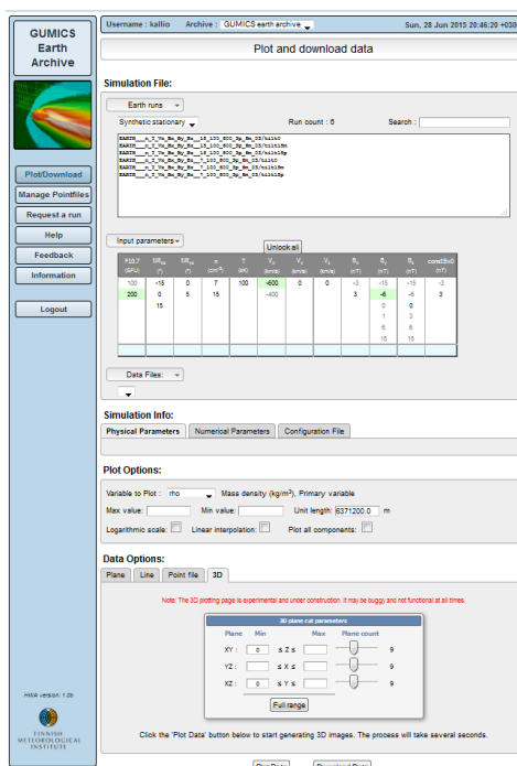
Figure 16: HWA ( http://hwa.fmi.fi/ ) MHD run catalogue, run access and search via input parameters.
