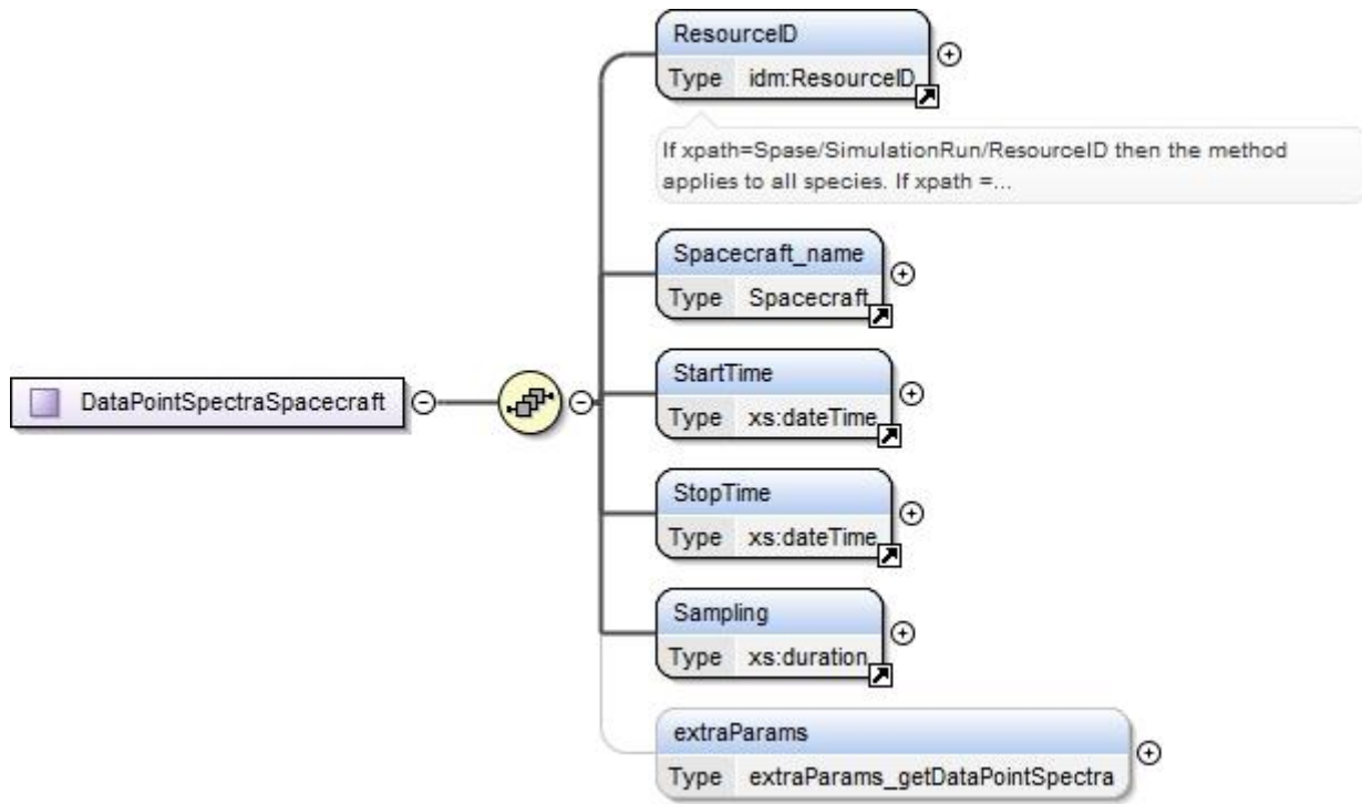
Figure 20: Schema of input parameters required for one web service.
