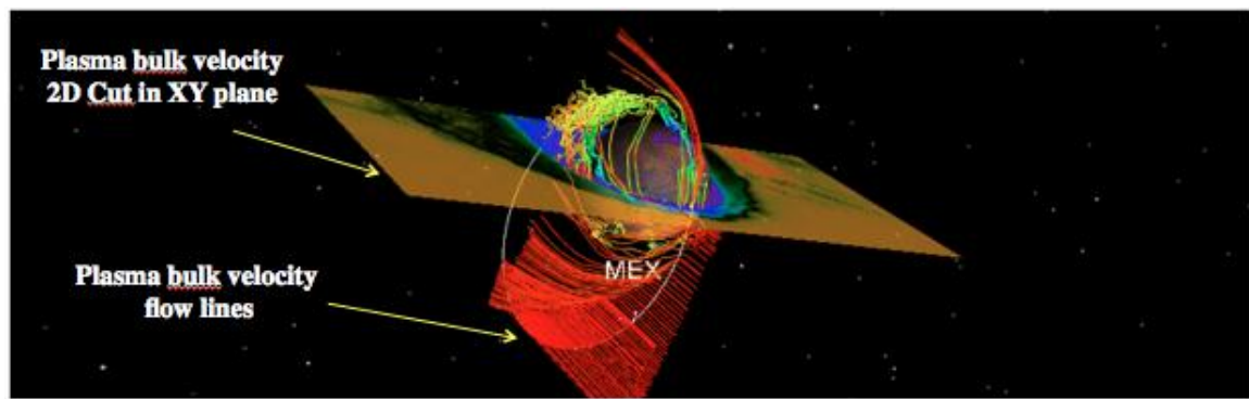
Figure 9: Display in CDPP-3DView of several types of simulation data around Mars (MEX). Hybrid model from LATMOS.
