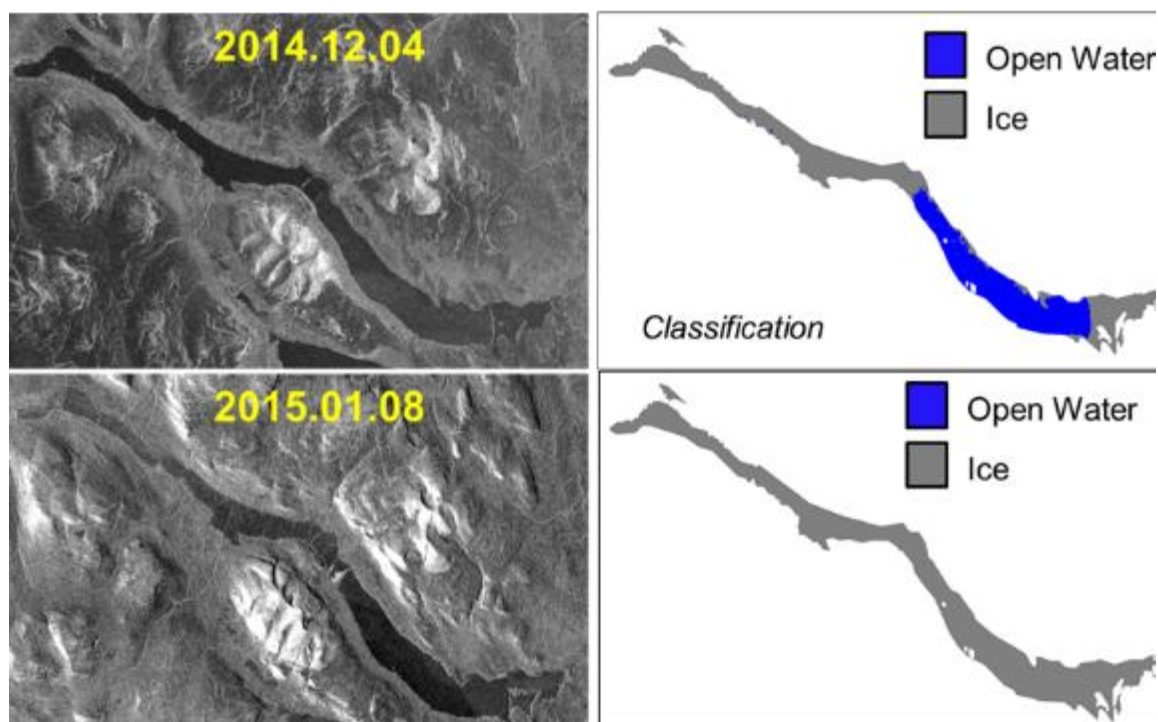
Figure 2.10: Sentinel-1A: Lake ice maps from Altevatn, Norway (Based on S1A VV-VH). The images are acquired during the lake ice formation period and during the polar darkness period in this region.
