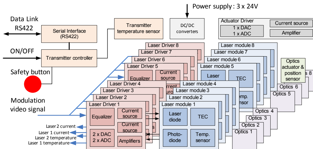
Figure 8 : transmitter block-diagram
