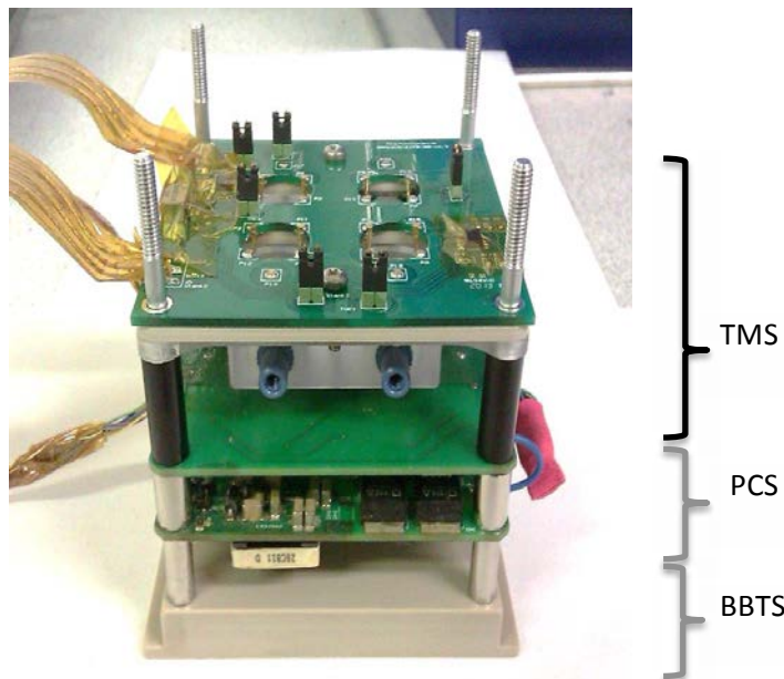
Figure 20: Picture of the MicroThrust BreadBoard System.
