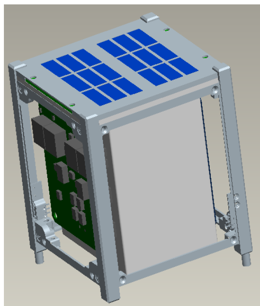
Figure 7: Propulsion system layout; MTS with long propellant tank and PCS boards placed along the sides
