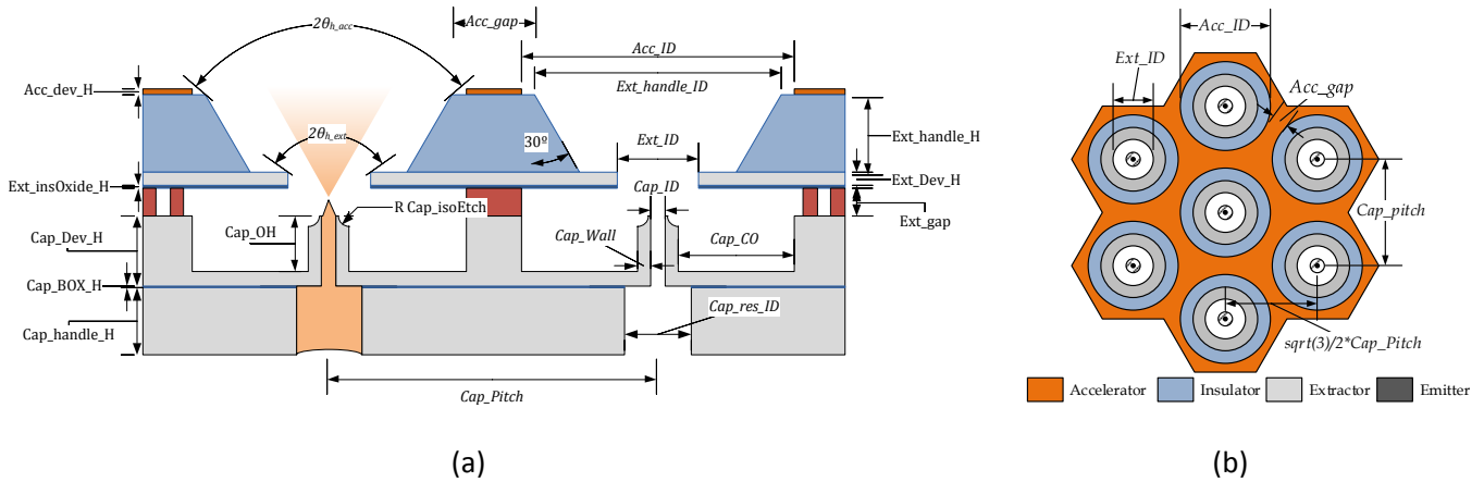
Figure 11: Cross-section (a) and layout (b) of the electrospray thruster array.
