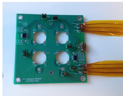
a) EIFB v1 with recesses for sealing PFIC & o-ring b) EIFB v2 (no clamping function)
