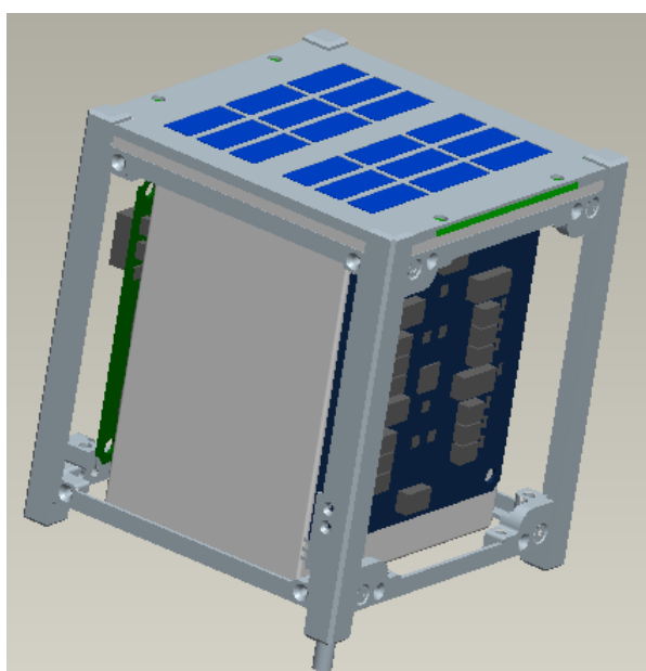
Figure 7: Propulsion system layout; MTS with long propellant tank and PCS boards placed along the sides
