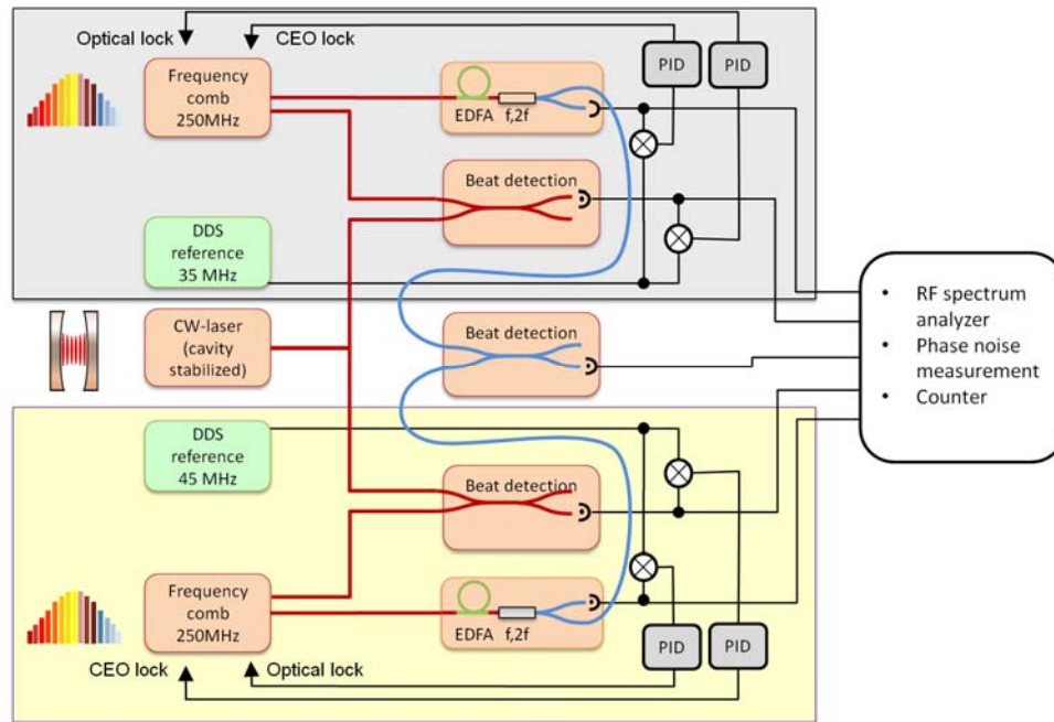
Figure 2.8: Setup for the figure-9 comb-comb comparison. Two frequency combs are locked to the same 1542 nm CW reference laser (left side, middle). The stabilization scheme is chosen such that the two optical frequency combs are offset by 10 MHz, sharing the same repetition rate. Temporally overlapping the two pulse trains on a photodiode, we observe the corresponding beat signal (center, middle).
