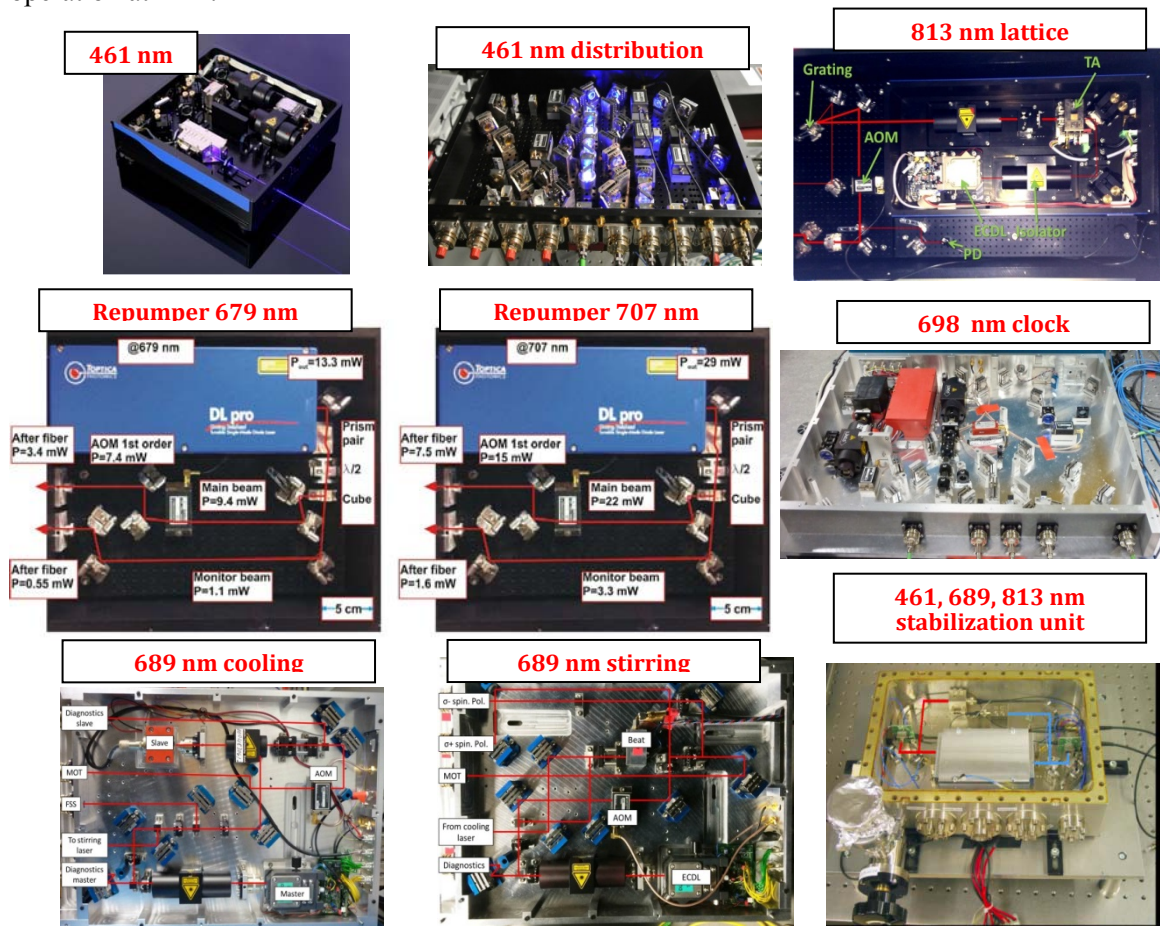
Figure 1.1 The laser subsystems for the 2 nd generation Sr clock apparatus.
