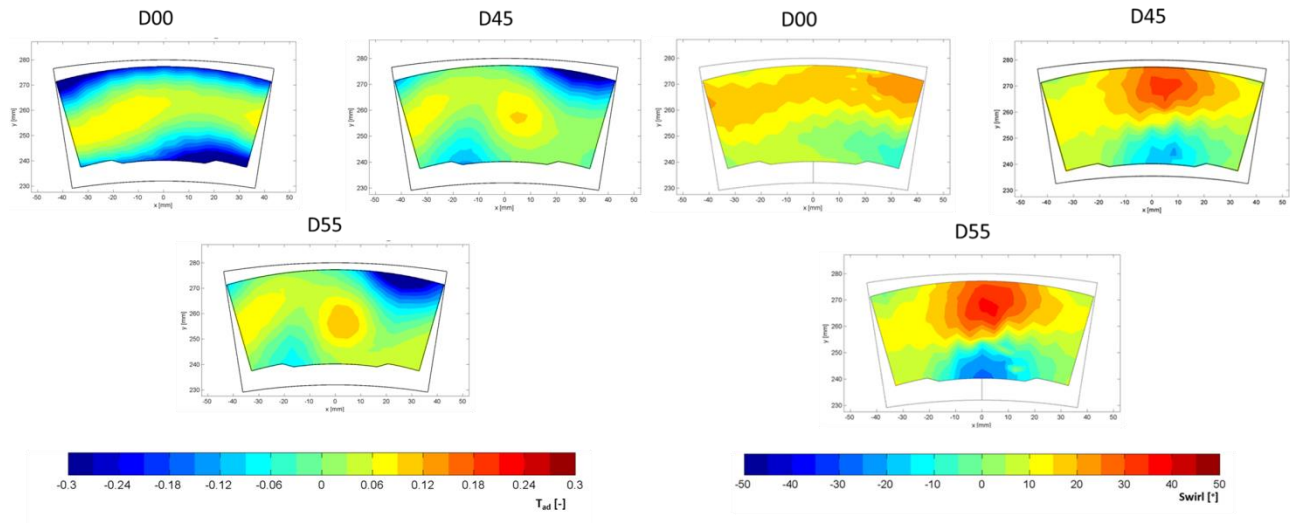
Figure 3: Temperature and swirl patterns on Plane 40+
