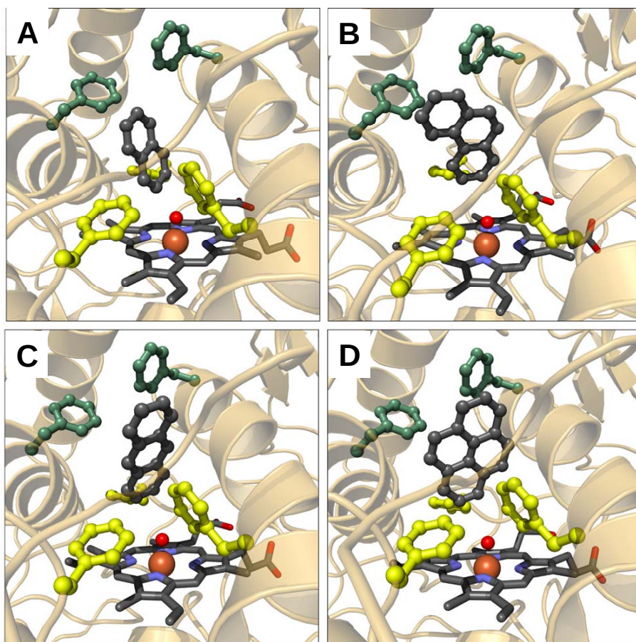
Fig. 2. A-D) Docking of naphthalene, phenanthrene, anthracene and pyrene substrates, respectively, on A. aegeirita UPO. Adapted from Piontek et al. (28).
