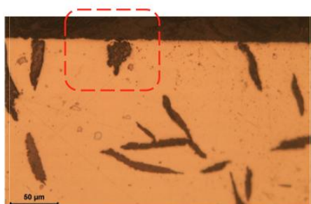
Closing of the open structure by superficial shear perpendicular to the sliding motion!
