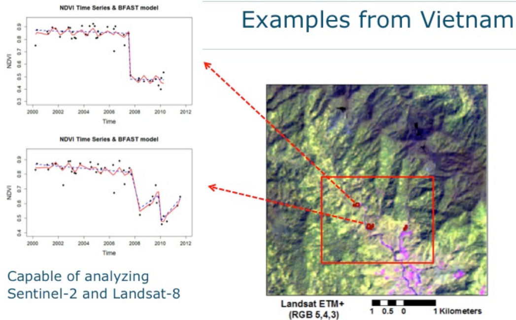
Fig. 1. Deforestation monitoring using satellite data in Vietnam using BFAST – Strucchange Marie Curie research developments.
