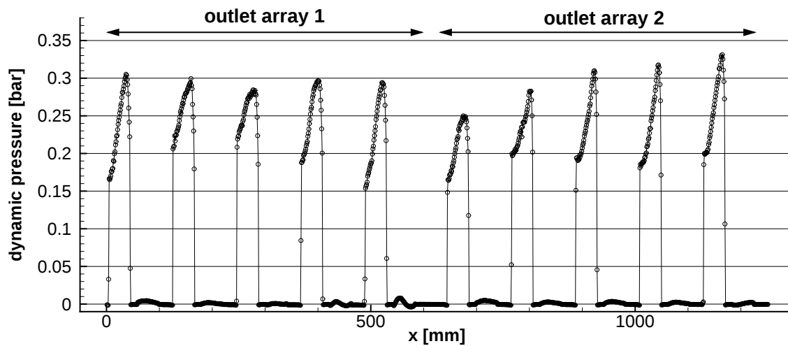
air jet exit profile for time step t_0 = 0\text{ms}
