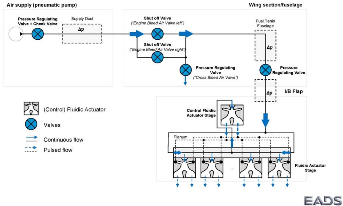
figure 6: system test rig (source EADS-IW)
