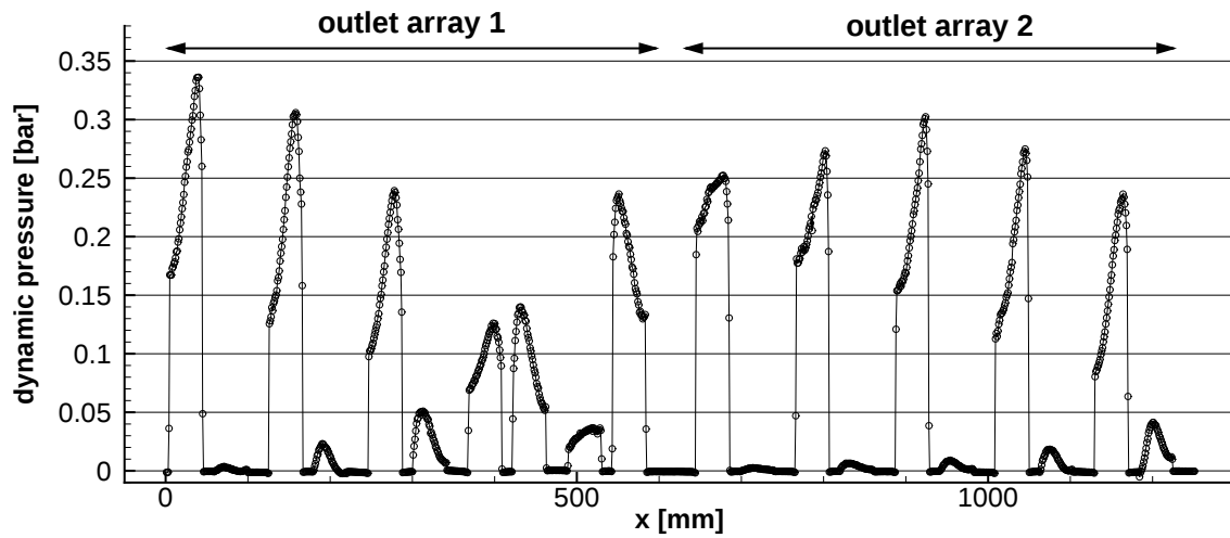
air jet exit profile for time step t_5 = 6.7\text{ms}
