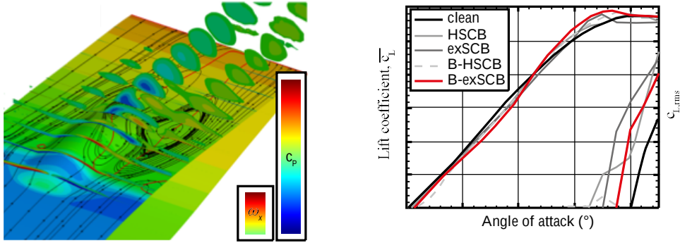
Figure 6: Computed skin friction lines, pressure contours and vorticity for HSCB in buffet; airfoil lift characteristics
