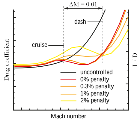
Figure 4: Polars comparing SCB performance with uncontrolled airfoil for various allowable cruise penalties
