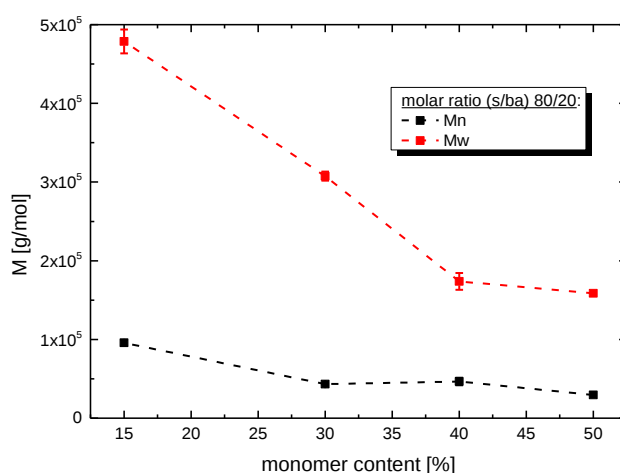
Figure 6: M_n and M_w for a molar ratio of 80/20 at different mass fractions monomer at isothermal conditions ( \tau = 12 min)
