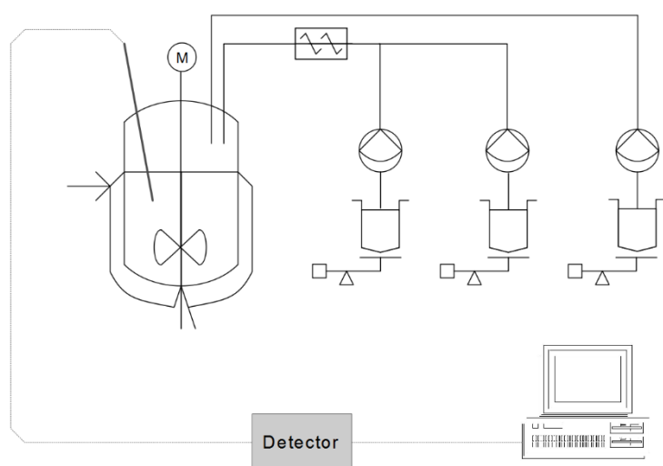
Figure 2: Semi batch set up UHAM
