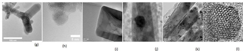
(g) CdS (h) ZnS (i) \text{Ca}_{10}(\text{PO}_4)_6(\text{OH})_2 (j) Ag inside sheet of \text{Ca}_{10}(\text{PO}_4)_6(\text{OH})_2 - scale bar is 5 nm (k) Pt on \text{TiO}_2 nanotubes (l) Ni MOF-74 - scale bar is 5 nm
