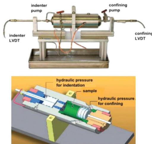
Figure 8: Experimental apparatus used for indentation tests
