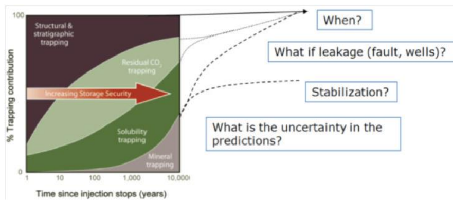
Figure 4: trapping diagram from IPCC 2005
