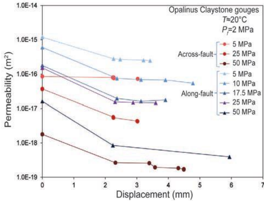
Figure 9: Fault permeability as a function of displacement for simulated clay-rich fault gouge prepared from crushed Opalinus Clay without leaching (see text). The permeametry experiments were performed at room temperature and a pore fluid pressure, P_f , of 2 MPa (argon gas).
