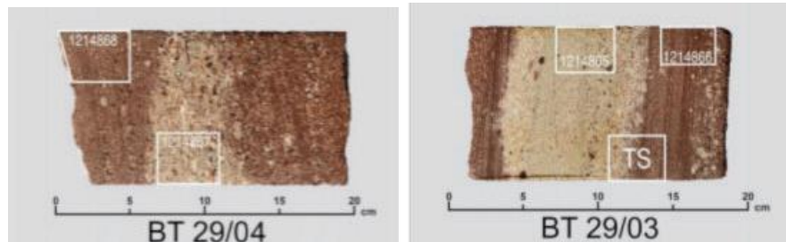
Figure 13: Example of thin sections from the site near Bad Teinach
