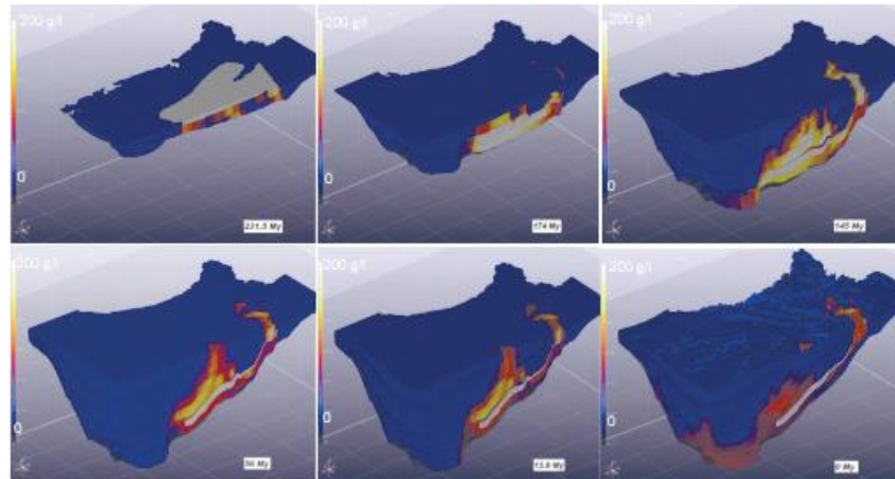
Figure 17: The modelling of the Paris Basin and the evolution of salinity simulated through geological time (million years, My). 3D view of the simulated salinity field through time (231.5 My, 174 My, 143 My, 56 My, 12.8 My, today (0 My)). Color scales range from 0 g/l (deep blue) to 200 g/l (white).
