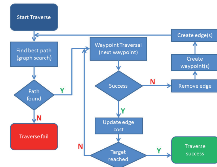
Figure 4: FASTER general operation scheme [Doc6.1]
