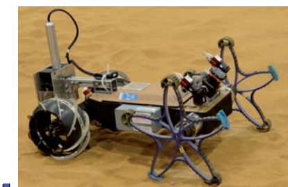
Figure 1: WLSIO system concept – wheel design [Doc4.1]
