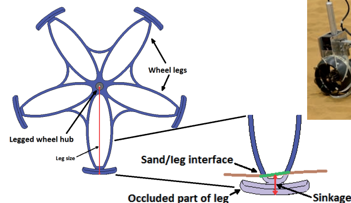
Figure 1: WLSIO system concept – wheel design [Doc4.1]
