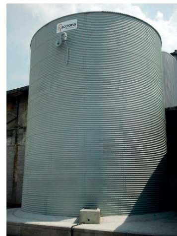
Photo 5. View of the STES in the Spanish Pilot Plant.
