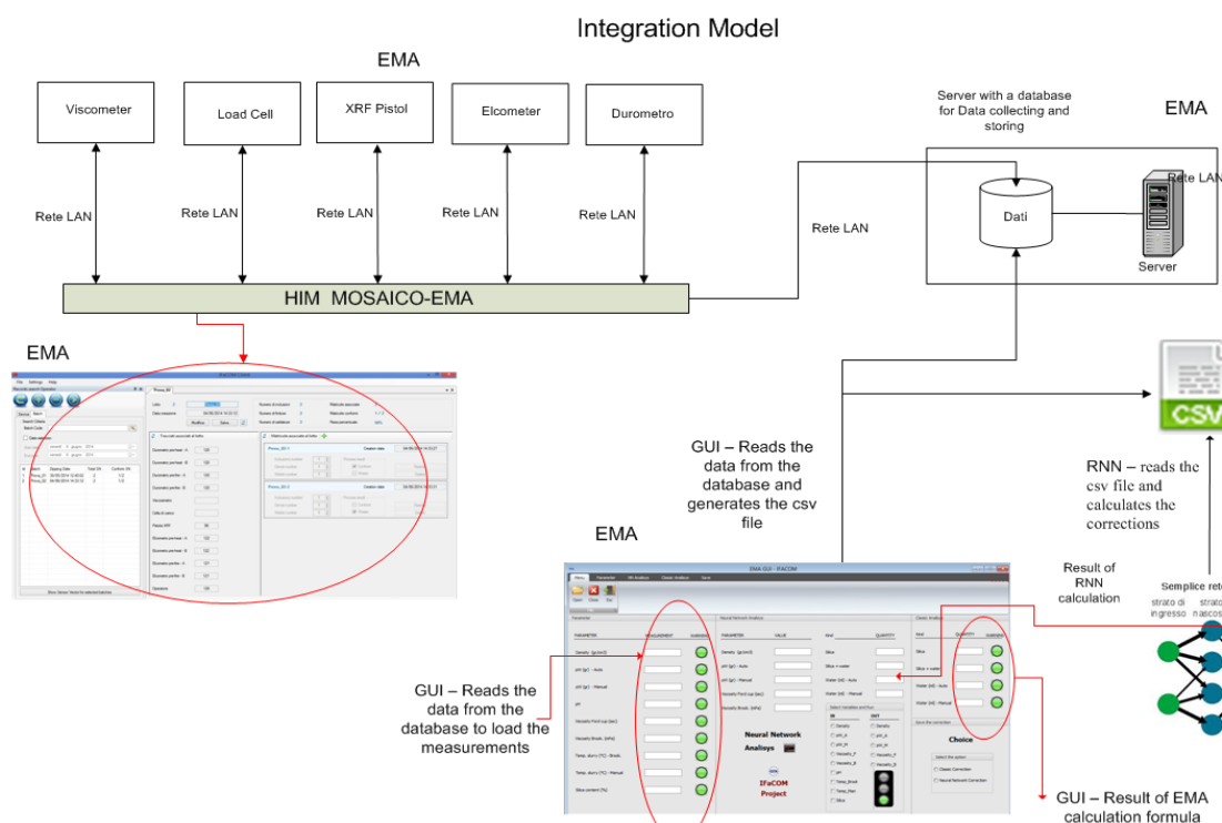
Figure 28: EMA's demo software architecture
