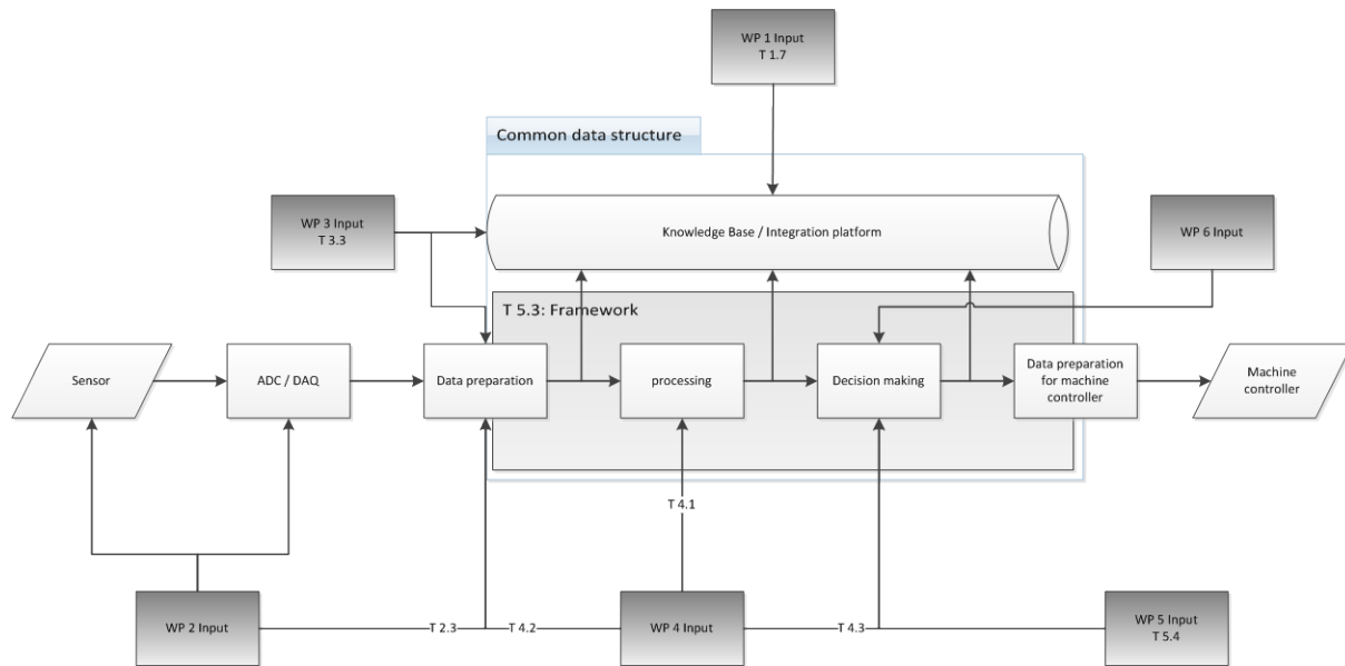
Figure 12: Data flow diagram of the IFaCOM-System
