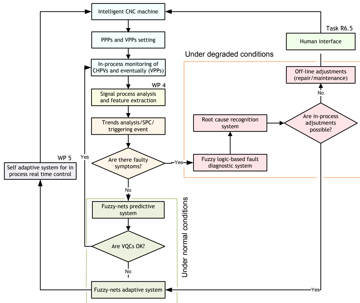
Figure 16: Main IFaCOM systems including the predictive and adaptive fuzzy-nets systems
