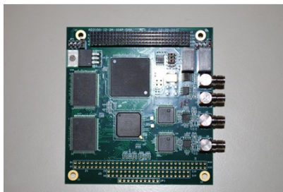
ACQUISITION BOARD
