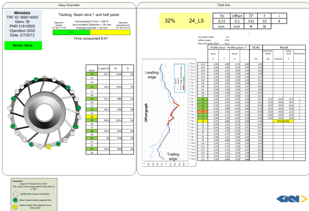
Figure 23: GKN's GUI
