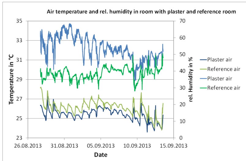
Figure 20: Temperature and relative humidity in Colegio El Porvenir
