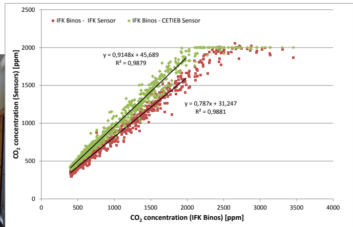
Figure 30: Left: Lesson room at University of Stuttgart for the \text{CO}_2 -monitoring. Right: Correlation of low cost sensors with analytical instrument. Values above 2000 ppm are only measured by the analytical instrument.
