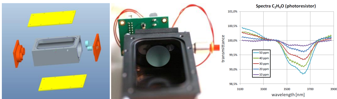
Figure 3: Left: Technical outline and view of the opened multi reflection cell. Right: Spectra series for Acetaldehyde from laboratory evaluation.
