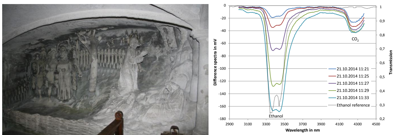
Figure 4: Left: Mount of olive relief which was treated. Right: Rise of ethanol concentration (difference spectra compared to spectrum before treatment). An Ethanol reference spectrum derived from IR data from NIST 2 is shown.
