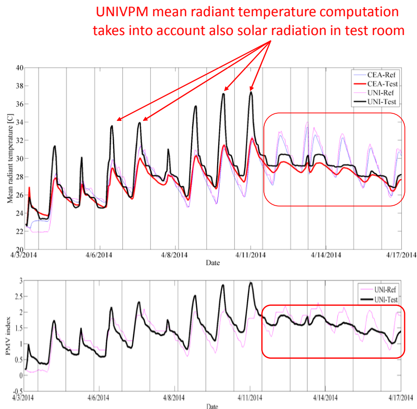
Figure 11: MRT and PMV in test room and reference room at CEA INES.
