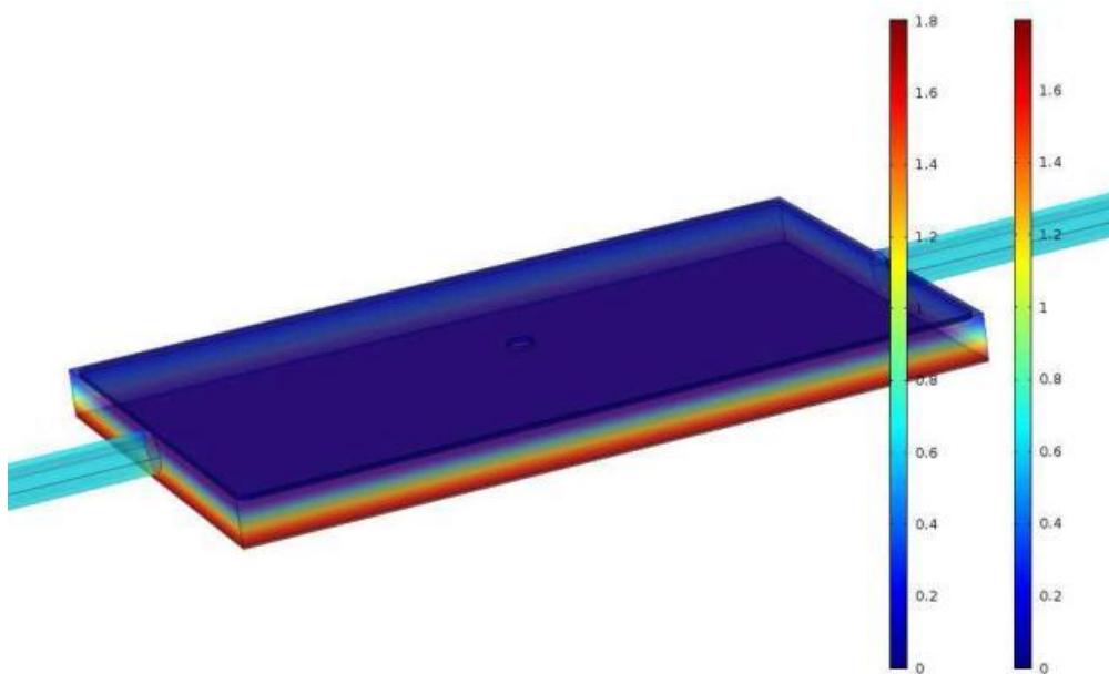
Figure 2: Electric field simulations
