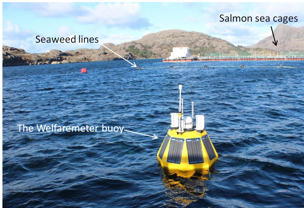
Figure 2: The Welfaremeter buoy deployed at a salmon and seaweed aquaculture site.
