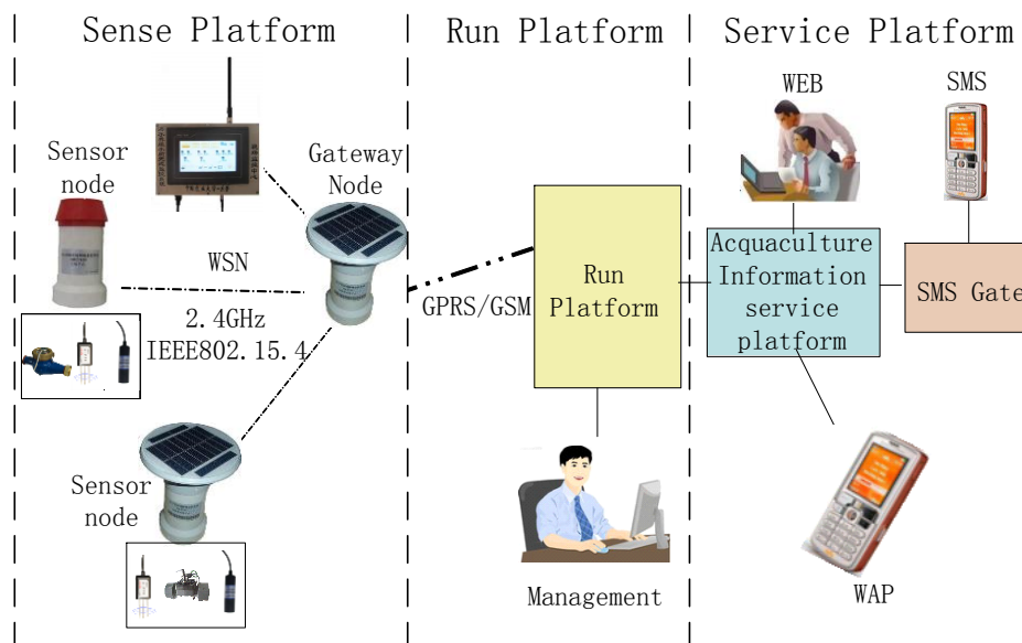
Fig. 3: Framework of aquaculture information system based on IoT
