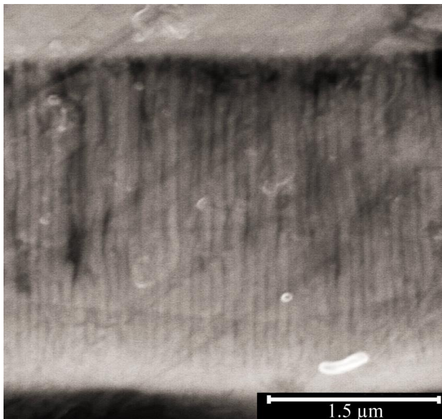
Illustration. Cross-sectional SEM micrograph of porous alumina template filled with zinc after two-stage electrochemical deposition.
