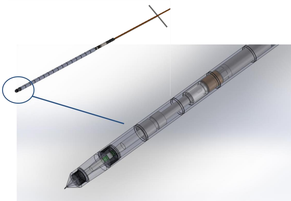
Figure 11: Schematic of the Proof of Concept of Spear System to measure profiles in sediments.
