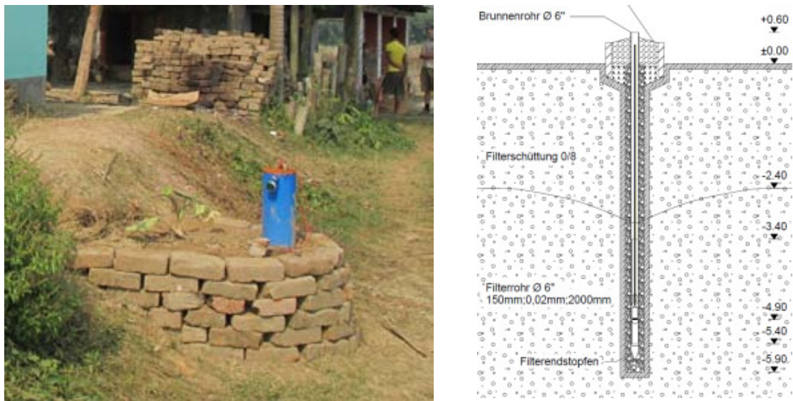
Figure 15: Protected head of well 1.
