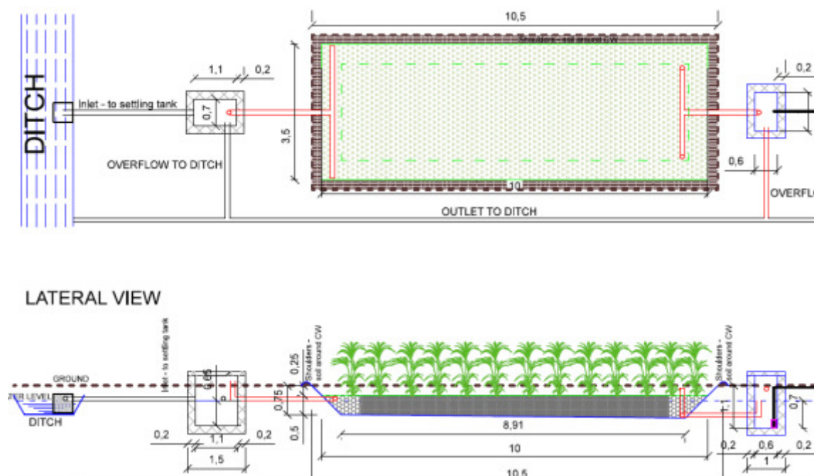
Figure 26: Design of planted gravel bed filter that has become necessary due to poor STP effluent quality.
