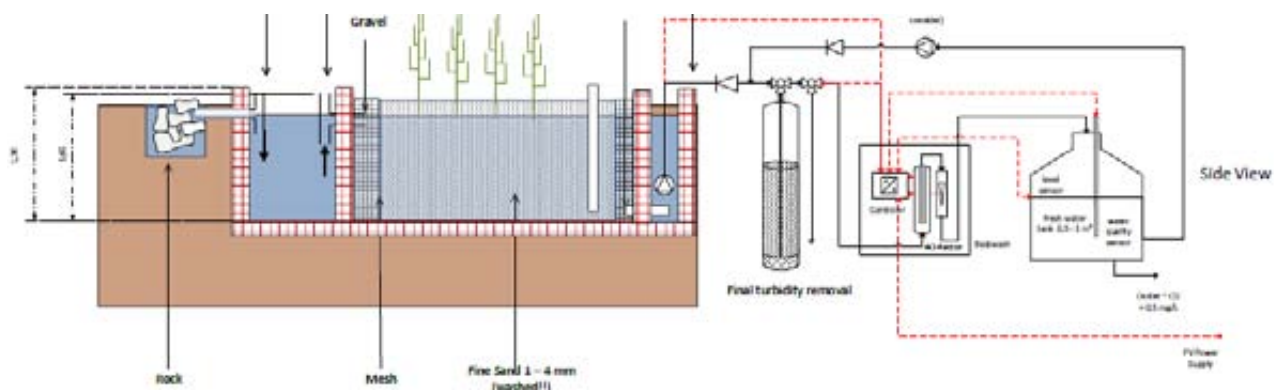
Figure 25: Original design of natural turbidity removal before AO disinfection at Amarkantak (IGNTU campus site).
