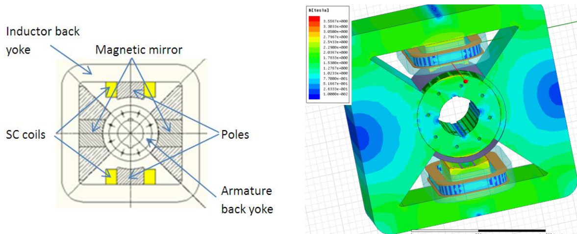
Figure 33. (left) SM electromagnetic layout (right) Magnetic field map of the SM
