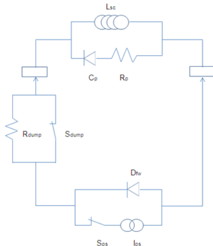
Figure 21. (Left) Quench protection scheme (Right) Stationary resistors bank
