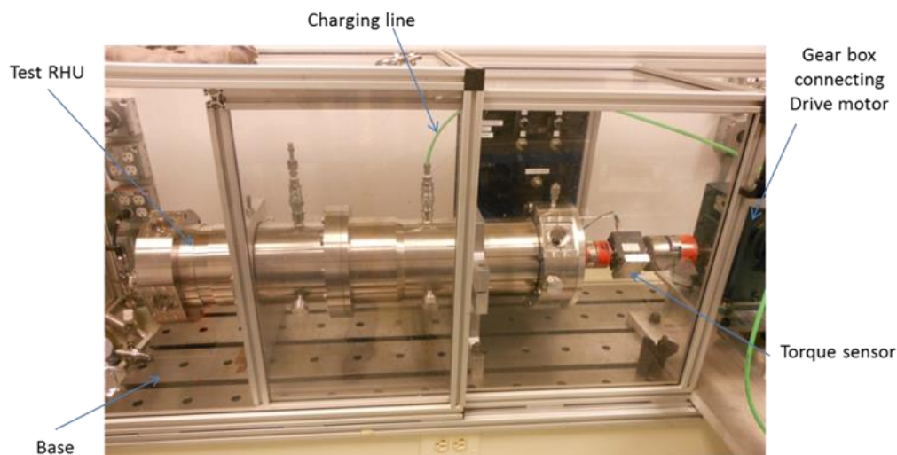
Figure 29. RHU under qualification tests
