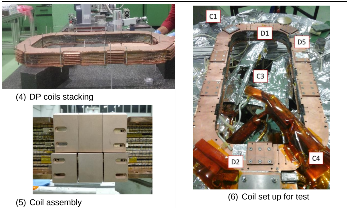
Figure 18. \text{MgB}_2 field coils manufacturing sequence
