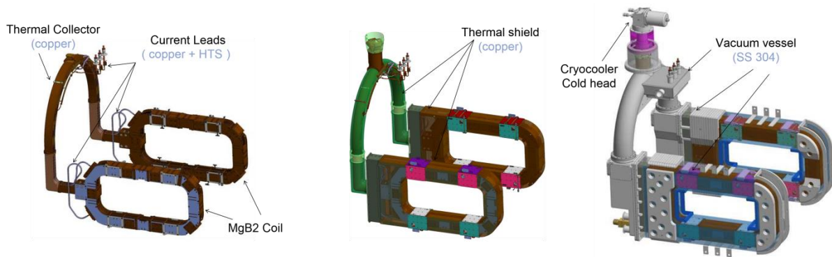
Figure 26. CAD model of the cryostat for the rotating magnetic validator
