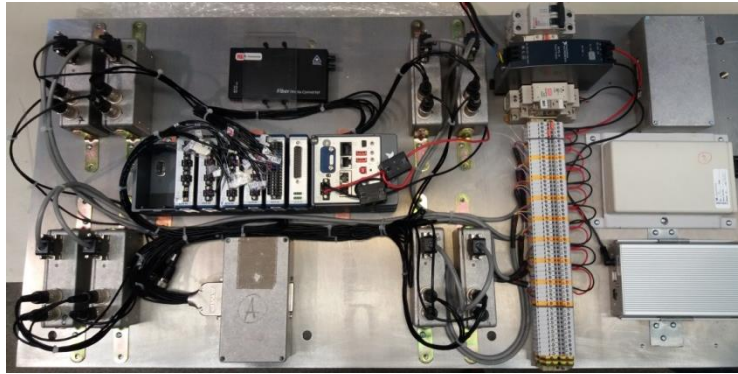
Figure 36. (left) stationary quench resistors (b) control hardware electrical panel Once manufactured all the elements next assembly sequence has been followed:
