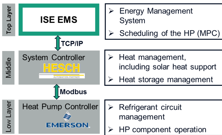
Figure 11 Controller hierarchy of the GreenHP project
