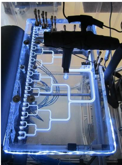
a) bionic plexiglass distributor b) cascade of venturi distributors c) nozzle distributor
