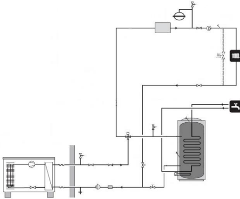
Figure 6: Indirect 3-pipe system
