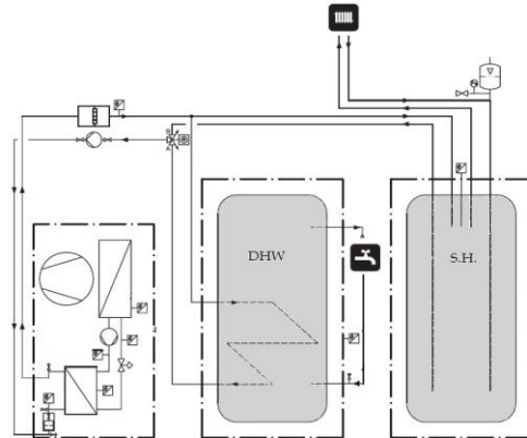
Figure 7: Indirect 4-pipe system
