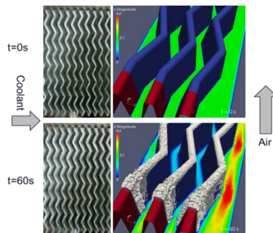
Figure 27: a) Icing Times and Heat Transfer for Various Fin Samples (Reichl 2015). Comparison Experimental / Numerical Studies (right) (Popovac 2015).
