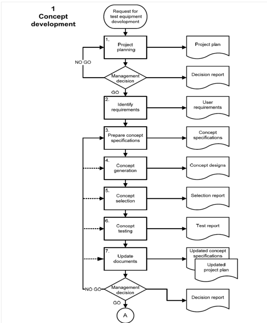
Fig. 15: Flowchart of the concept development phase
