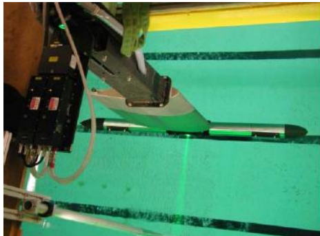
Fig. 1: Integrated light sheet probe
