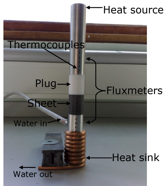
Figure 7: Axial heat flow apparatus to measure the TCC between two polymeric materials
