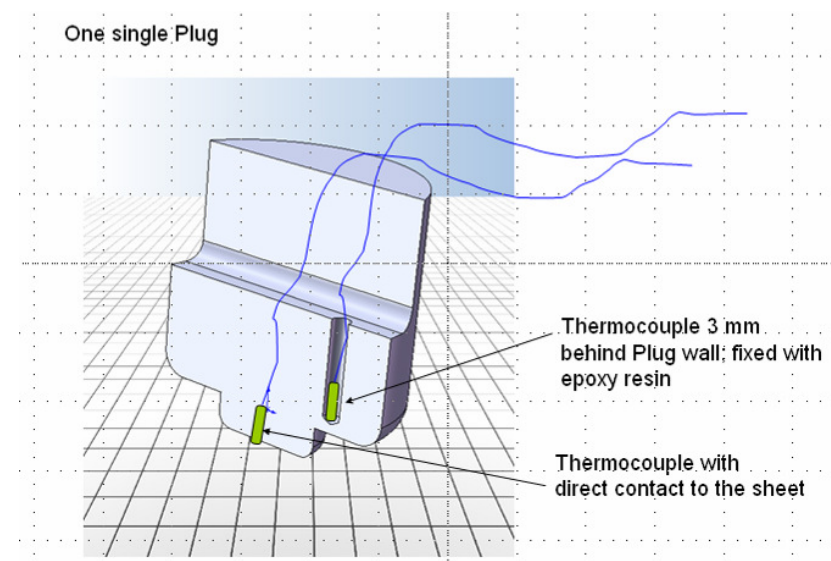
Figure 14: Drawing of a single plug with sensors inside
