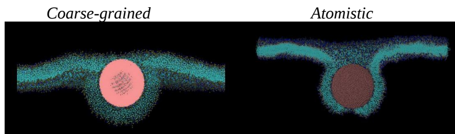
Fig. 16: CG simulation of the system in figure 15 (10 nm Au particle) without matching the bending modulus. The join at the NP is not the same in the two simulations.
