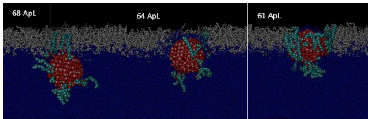
Fig. 10: In atomistic simulations where the NP/lipid interaction is stronger than the NP/water interaction the lipid head groups bind the NP to the headgroup layer. Illustrated here for a water-supported monolayer DPPC layer at three different physiological areas per lipid (ApL), [ \text{\AA}^2 ].
