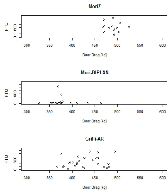
Figure 1. Comparison of sediment resuspension (FTU) against the advance resistance (drag) for a traditional otterboard (MoriZ) used as a reference, and two innovative otterboards (Mori-BIPLAN and Grilli-AR).
