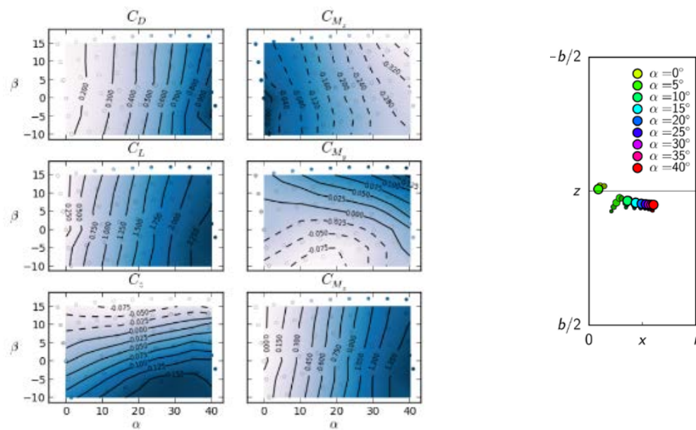
Figure 11. Analysis of data collected from wind tunnel tests. The picture on the left shows the drag coefficient ( C_D ), the spread coefficient ( C_L ) and the lift coefficient ( C_z ), the momentum coefficients ( CM_x, y, z ), against the attack angle ( \alpha ) and roll angle ( \beta ). On the right the position of the centre of pressure for different attack angles.
