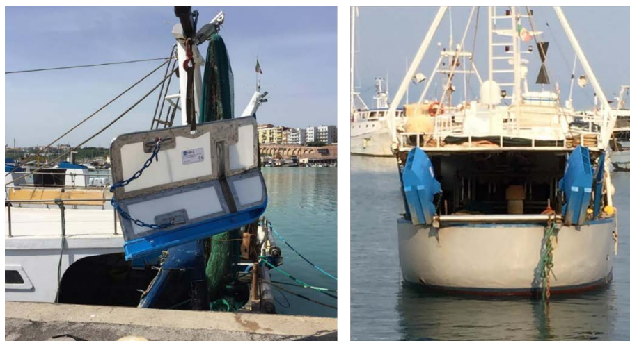
Figure 12. Novel otter-boards developed within the project BENTHIS. On the left Grilli-AR, on the right Mori-BIPLAN.
