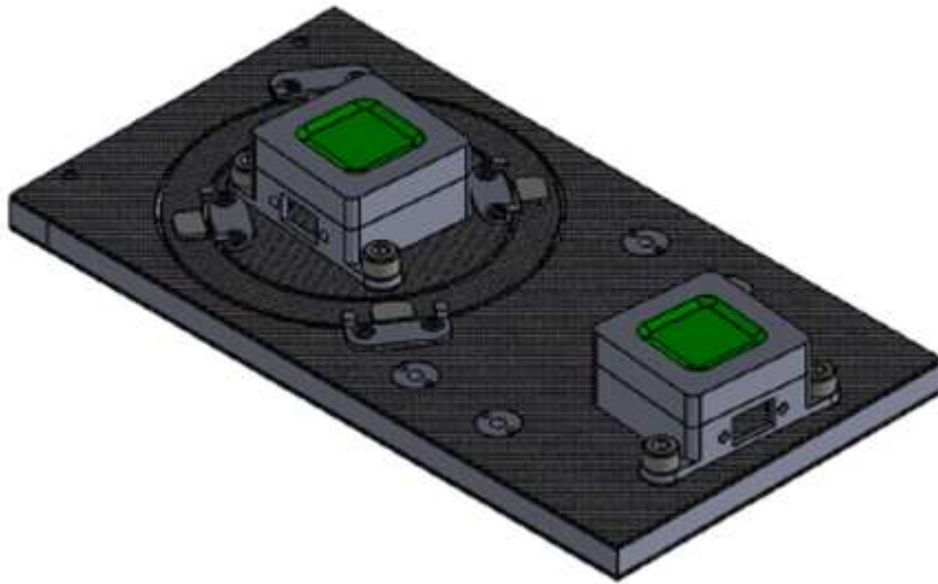
Figure 1, Design drawing of the Smart Structure with a fixed sun-sensor and a second sun-sensor mounted on a gimballed structure that can be tilted by means of 2 piezo bimorph actuators located at the back side of the panel
