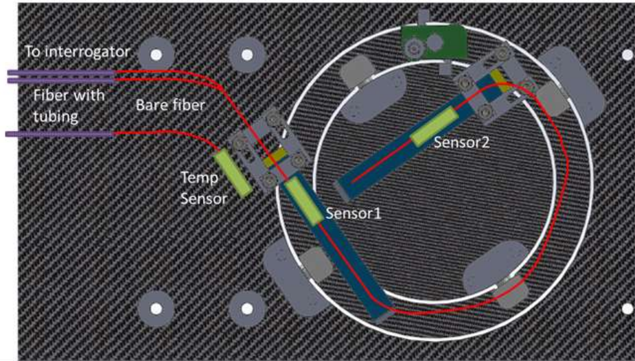
Figure 2, design drawing of the back side of the smart panel showing the 2 piezo beams that tilt the gimballed ring and disc. On the surface of the two piezo beams strain is measured by means of FBG sensor gratings that make use of a single fiber.
