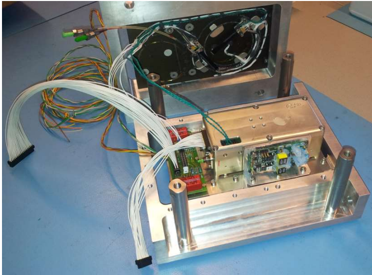
Figure 3, space compatible miniature interrogator (110 x 50 x 40 mm aluminum box) mounted in a test frame. The back side of the smart panel mounted in a separate test frame is also visible
