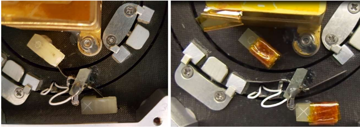
Figure 4, launch-lock for the smart panel based on an SMA beam that blocks the gimballed ring and disc during launch (left). When heated the SMA beam returns to its pre-programmed S-shape releasing the lock (right)
