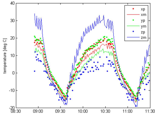
Figure 6, measured temperature of the solar panels on the satellite sides: x, y and z of the satellite (p and n side) as a function of time. The graph shows the slow temperature change resulting from the eclipse in the ~100 minute orbit cycle and the faster temperature changes related to tumbling of the satellite.
