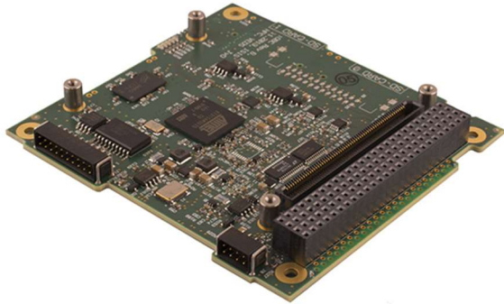
Figure 7, Generic Cubesat Payload Data Acquisition Unit (PDAU) developed for offloading the On Board Computer (OBC) from payload specific processing tasks.
