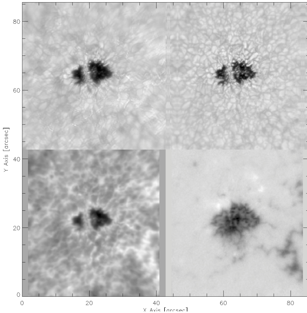
Some sample images from the Active Region test data-set. Upper-left: G-band image; Upper-right: Broad-band image; Lower-left: Stokes-I image near the core of the FeI 617.3 nm line; Lower-right: Stokes-V image near the wing of the FeI 617.3 nm line. For the sake of visualization, all images have been rescaled to the same pixel resolution ( 0.167 \text{ arcsec pixel}^{-1} ), their values have been separately linearly scaled to saturate the greyscale palette and we only show the central part of the Broad-band and spectropolarimetric images.
