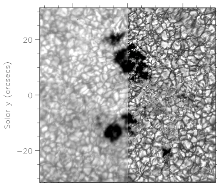
A solar image from ROSA. The right half of the image has been reconstructed with the KISIP speckle code.
