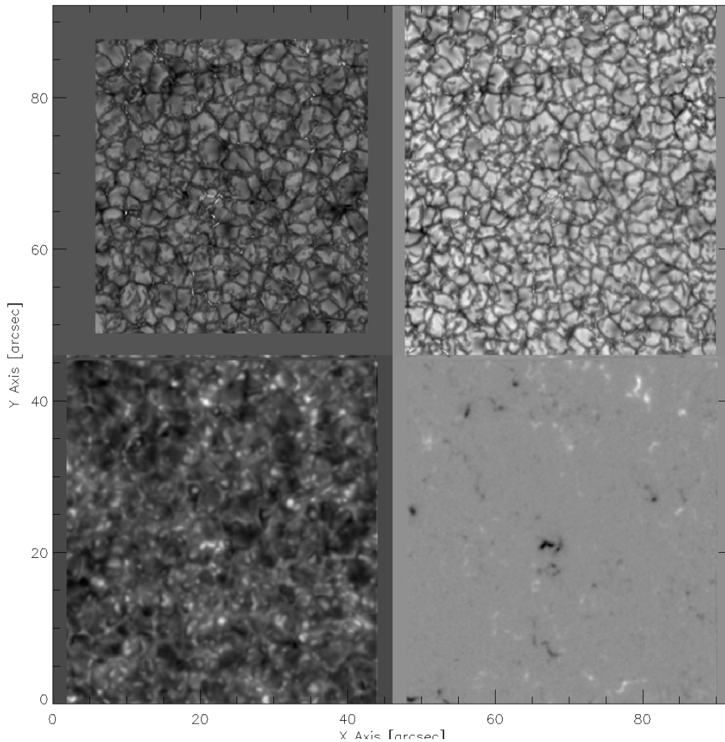
Sample images from the Quiet Sun test data-set. Upper-left: G-band image; Upper-right: Broad-band image; Lower-left: Stokes-I image near the core of the FeI 630.2 nm line; Lower-right: Stokes-V image near the wing of the FeI 630.2 nm line. For the sake of visualization, all images have been rescaled to the same pixel resolution ( 0.18'' \text{ pixel}^{-1} ) and their values have been separately linearly scaled to saturate the greyscale palette.
