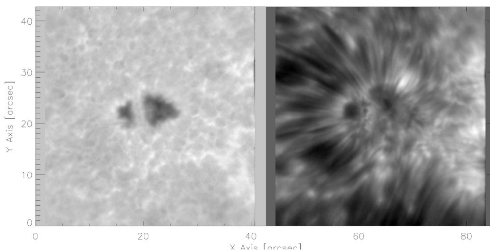
Sample images from the chromospheric data-set data-cubes. Left: Stokes-I image near the wing of the Ca II 854.2 nm line; Right: Stokes-I image near the core of the Ca II 854.2 nm line. For the sake of visualization, we only show the central part of the images and their values have been separately linearly scaled to saturate the grey-scale palette.
