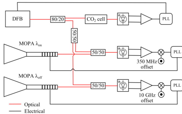
Fig. 10: Schematics of the Frequency Stabilization Unit (FSU).
