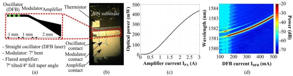
Fig. 7: Fabricated 3-section bent MOPAs. (a) Schematics of the device. (b) Photograph of the device. (c) Power vs PA current characteristics at T = 18^\circ\text{C} . (d) Optical spectrum while varying the DFB current.
