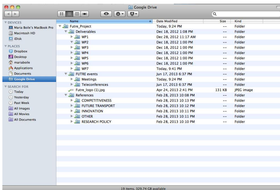
Figure 16-Workspace structure
