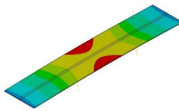
b) Intermediate welds: 400 rpm – 325 mm/min
