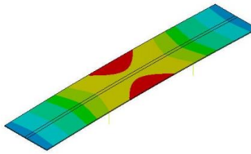
a) Slow welds: 200 rpm – 175 mm/min
