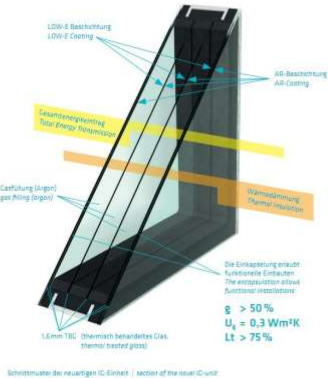
Figure 3: pattern of quadruple IG-Unit
