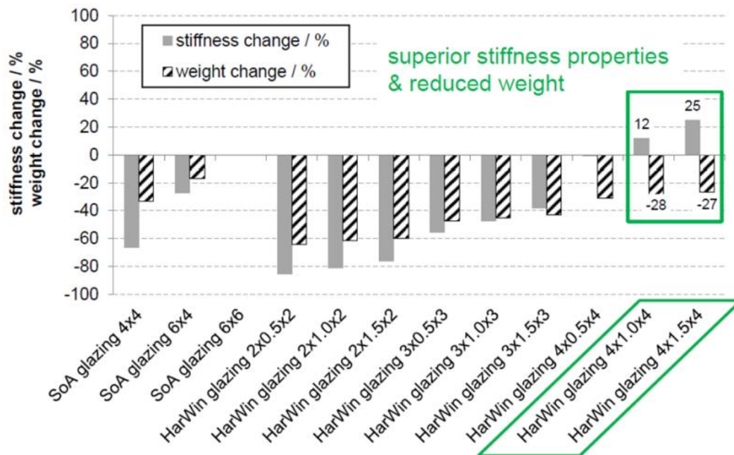
Figure 2.1-4.: Comparison of the results of simultaneous improvement of mechanical properties and weight reduction for HarWin glazing panes relative to state of the art 6x6 mm 2 laminated glazing. Description: 4x0.5x4 means two 4 mm glass panes laminated with 0.5 mm of softener containing PVB-glass-flake composite.
