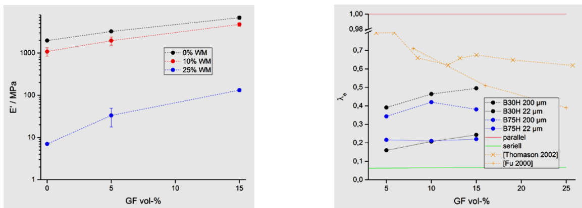
Figure 2.1-3.: left: Storage moduli (at 25°C) as a function of glass flake and softener (WM, Weichmacher) content of a PVB-glass flake composite interlayer measured by means of dynamic mechanical analysis; right: efficiency factor for stiffness increase upon glass fiber addition as compared to glass flake addition
