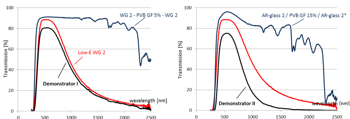
Figure 2.2.-1.: Transmission spectra of double (Demonstrator I) and triple glazing (Demonstrator II)
