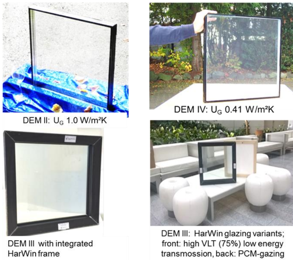
Figure 2.: HarWin Demonstrator glazing variants and windows with glazing 500x500 mm 2
