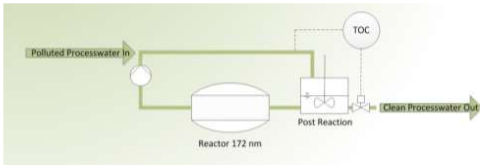
Fig. 2: L4CW-Demo Process Scheme
