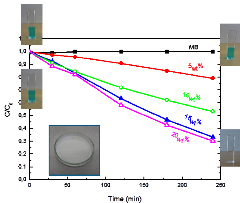
Photocatalytic activity of PMMA/TiO 2 films with 5 wt % NPs (full dots), with 10 wt % NPs (open dots), with 15 wt % NPs (full triangles) and with 20 wt % NPs (open triangles) compared to the discoloration of pure MB under UV illumination (squares). Inset: PMMA/TiO 2 films with 15 wt % NPs in the Petri dish.
