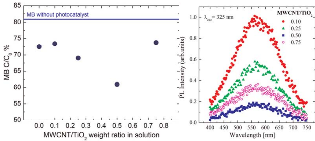
(a) Residual percentage of the initial MB concentration ( C_0 ) calculated from the 664 nm absorbance peak for different MWCNT/np-TiO 2 composites. The blue line shows the residual C/C_0 value of MB after irradiation without the photocatalytic sample; (b) Photoluminescence spectra of the samples with MWCNT/TiO 2 ratio= 0.10, 0.25, 0.50 and 0.75. The excitation wavelength is 325 nm.
