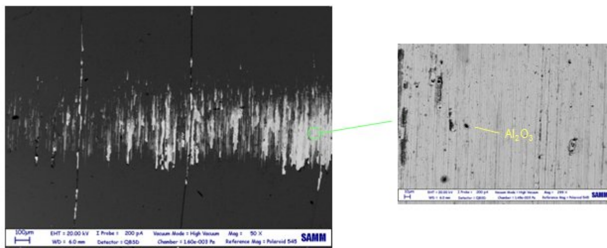
Figure 3-6: Results on surface optical analysis: Nitr.+Cr+DLC vs. Cr in water with \text{Al}_2\text{O}_3
