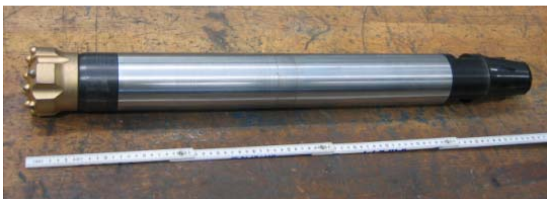
Figure 3-18: 3 ¼ inches DTH STREAM prototype
