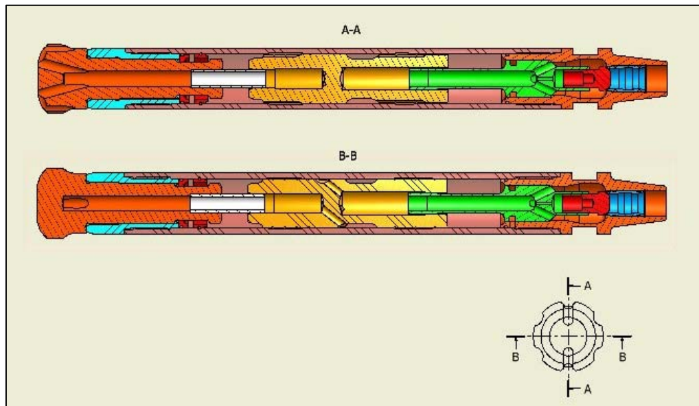
Figure 3-9: Model of the pneumatic DTH hammer
