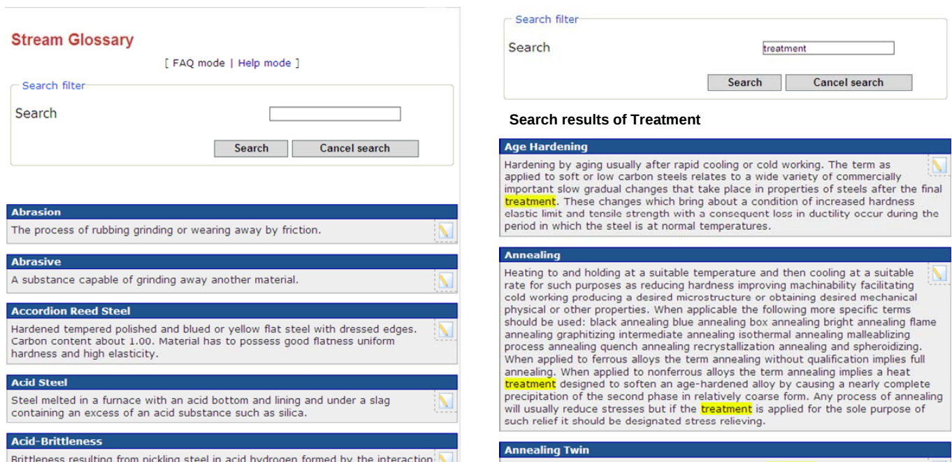
Figure 3-3: STREAM Glossary
