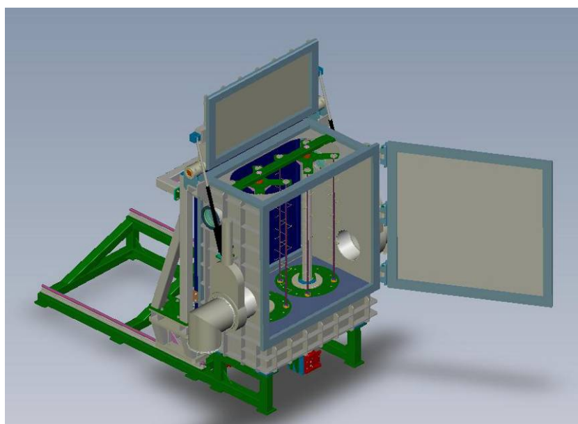
Figure 3-5: Design of the industrial DLC deposition plant with 1,0 \times 1,0 \times 0,7 \text{ m}^3 coating volume area
