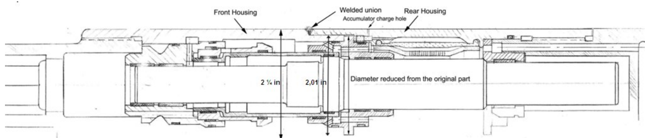
Figure 3-22: 2D drawing of the 2 ¼ inches prototype
