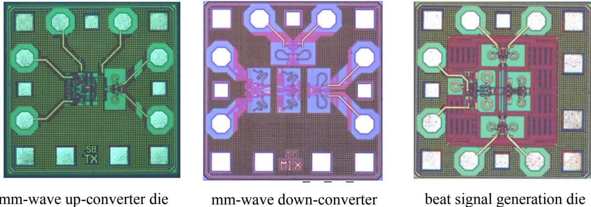
Figure 3-12: Micrographs of the active key components of the mm-wave up-down converter.
