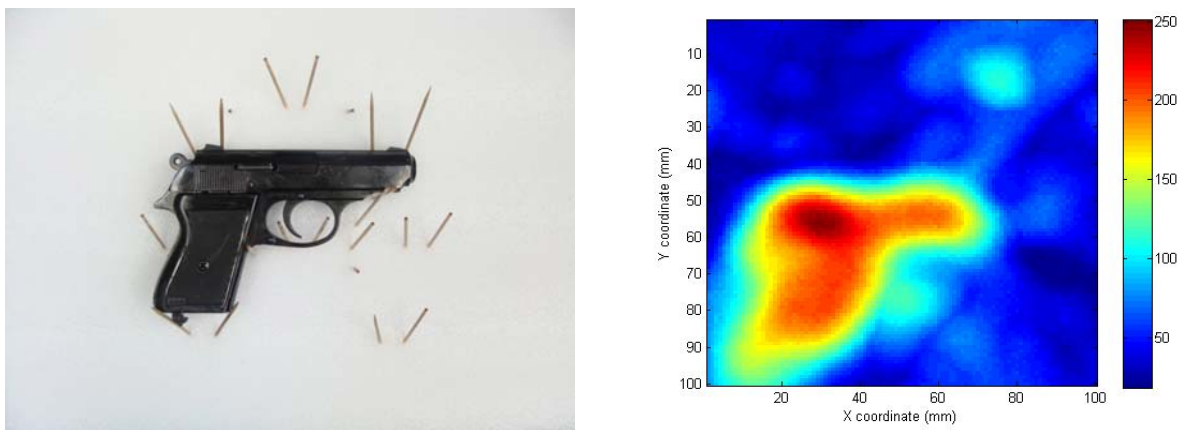
Figure 3-21: MIMO imaging of a gun in frequency band 3.1 -10.6 GHz.
