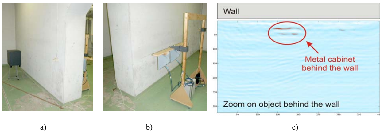
Figure 2-30: Through 60 cm concrete wall SAR scanning: a) Metal cabinet behind the wall, b) Scanning system, c) Imaging and detection of metal cabined behind 60 cm concrete wall
