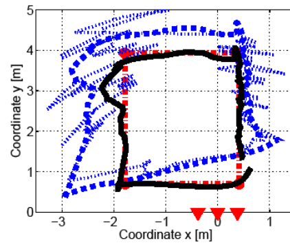
Figure 2-26: Scenario Concrete-1d: target trajectory estimations.
