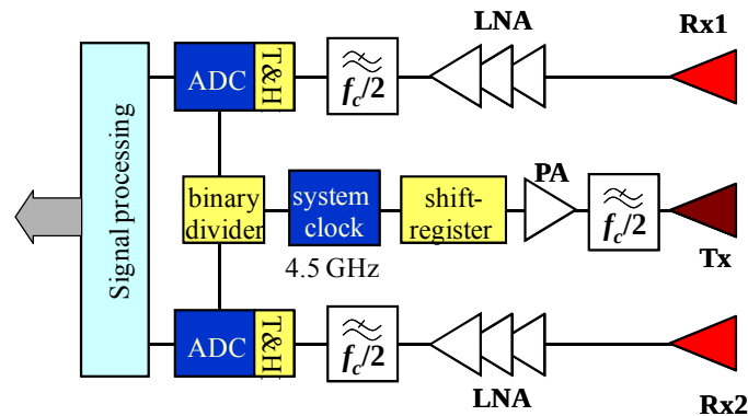
Figure 4-3: Block schematics of the radar device
