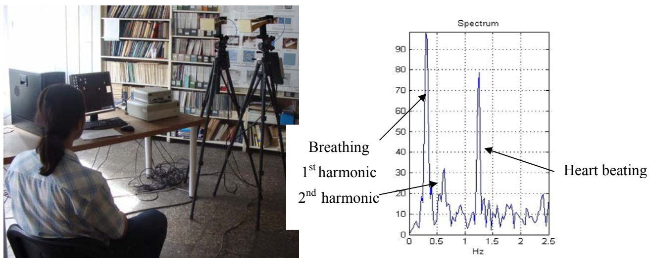
Figure 4-13: Breathing and heart beating spectrum measurement in frequency band 1 -30 GHz
