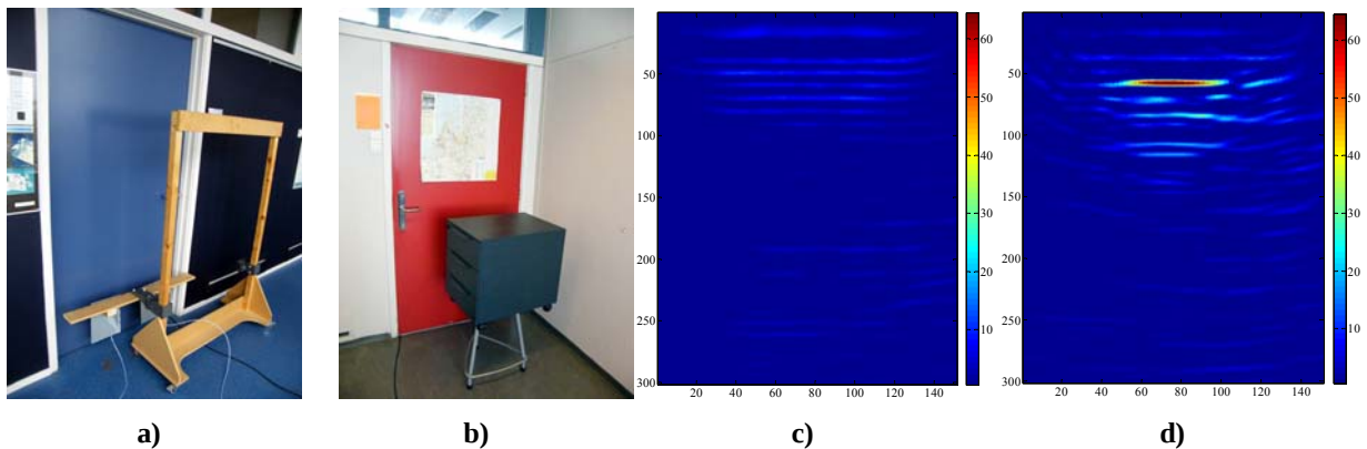
Figure 2-29: Through door SAR scanning: a) Scanning system, b) Metal cabinet behind the door c) Imaging of empty room, d) Imaging of metal cabined behind the door
