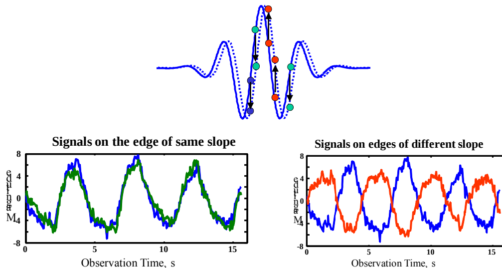
Figure 4-2: Simplified shape of a backscattered signal and the voltage variation of different samples due to a small shift of the target (above). Measured voltage variation of some samples due to breathing of a person (below).
