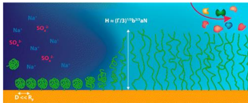
Figure 2. Principle schematic of grafting and protein resistance of poly(ethylene glycol) brushes. The images is the table of content graphic for the publication in ACS Applied Materials and Interfaces 2015.
