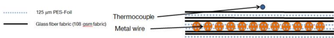
Figure 13 Final layout of separation layer
