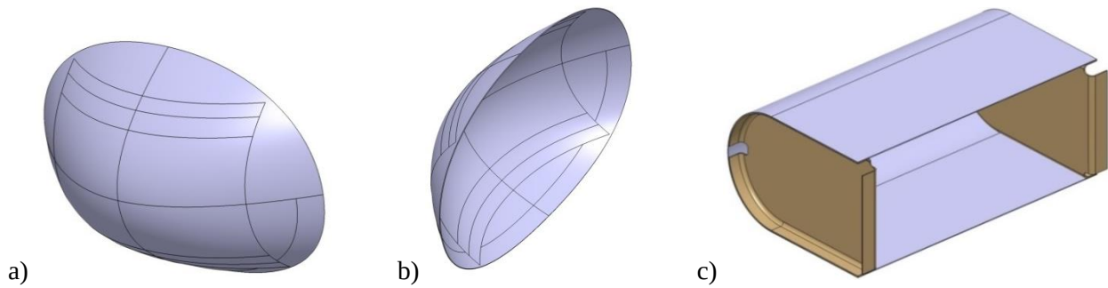
Figure 4 Planed demonstrators for the GRC6.2 Project (ECO-Fairs): a) and b) Radom; c) sponson fairing (AW)
