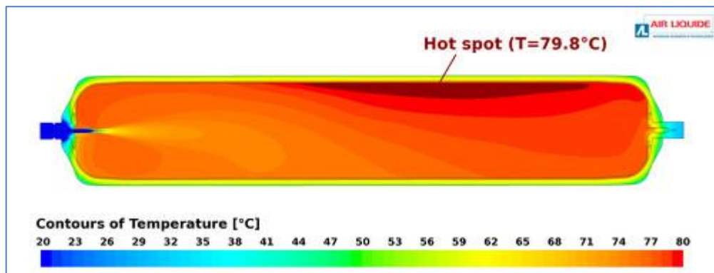
Figure 5 CFD simulation of the filling of a 531 litre hydrogen tank with hydrogen at -20°C for 25 minutes. As one result, thermocouples for recording temperature during experiments were placed according to this temperature field. Source: Air Liquide-aT / HyT 2014
